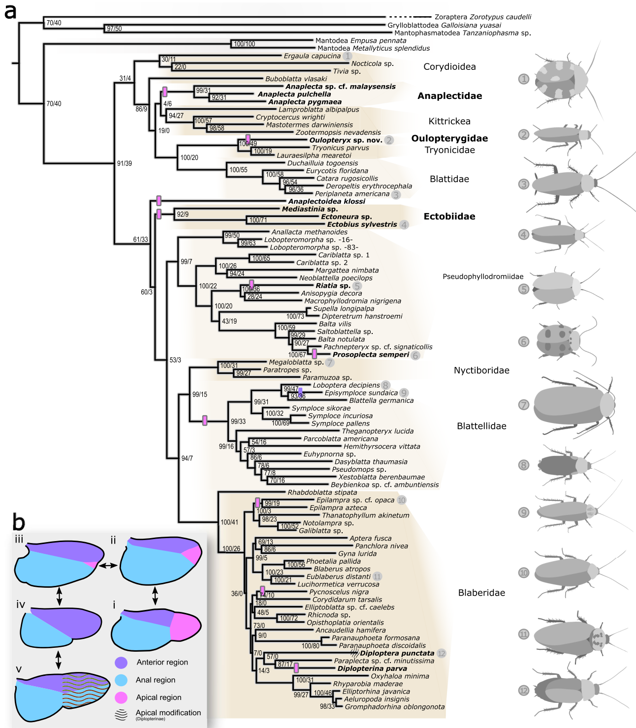
Fig. 1 Phylogeny of Blattodea (a) and wing morphology illustration (b). a The phylogeny presented is the final species tree resulting from a number of topology tests and inference methods (IQ-TREE and ASTRAL). Node support values represent bootstrap frequency (3000 replicates from concatenation analyses of all three modified alignments; left) and gene concordance factors among the 41 loci (right). Taxa in bold have hind wings with a very large apical folding area (b – i, and b – ii). The apical region in Diploptera may not be homologous to those of other taxa so we use another symbol and did not count them as addi-
