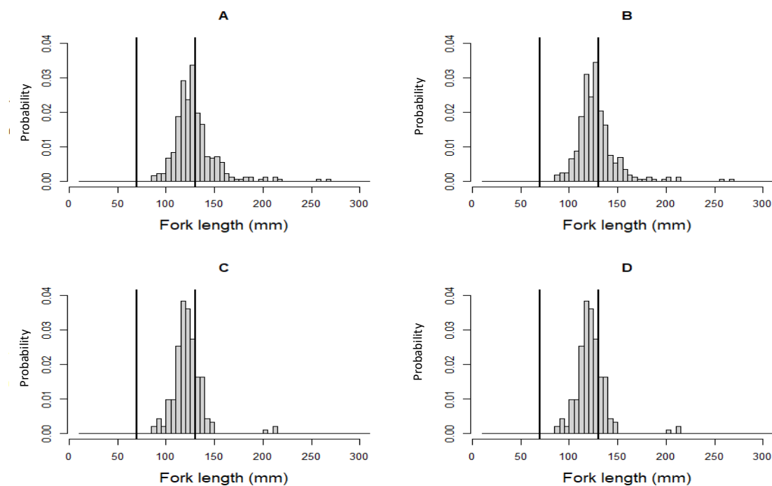
Figure 9: Histogram of fork length A: with no filter ( N = 363 ); B: with a Range less than 6 meters ( N = 343 ); C: with a Precision less than 10% ( N = 182 ); D: with a Range less than 6 meters and a Precision less than 10% ( N = 182 ).
