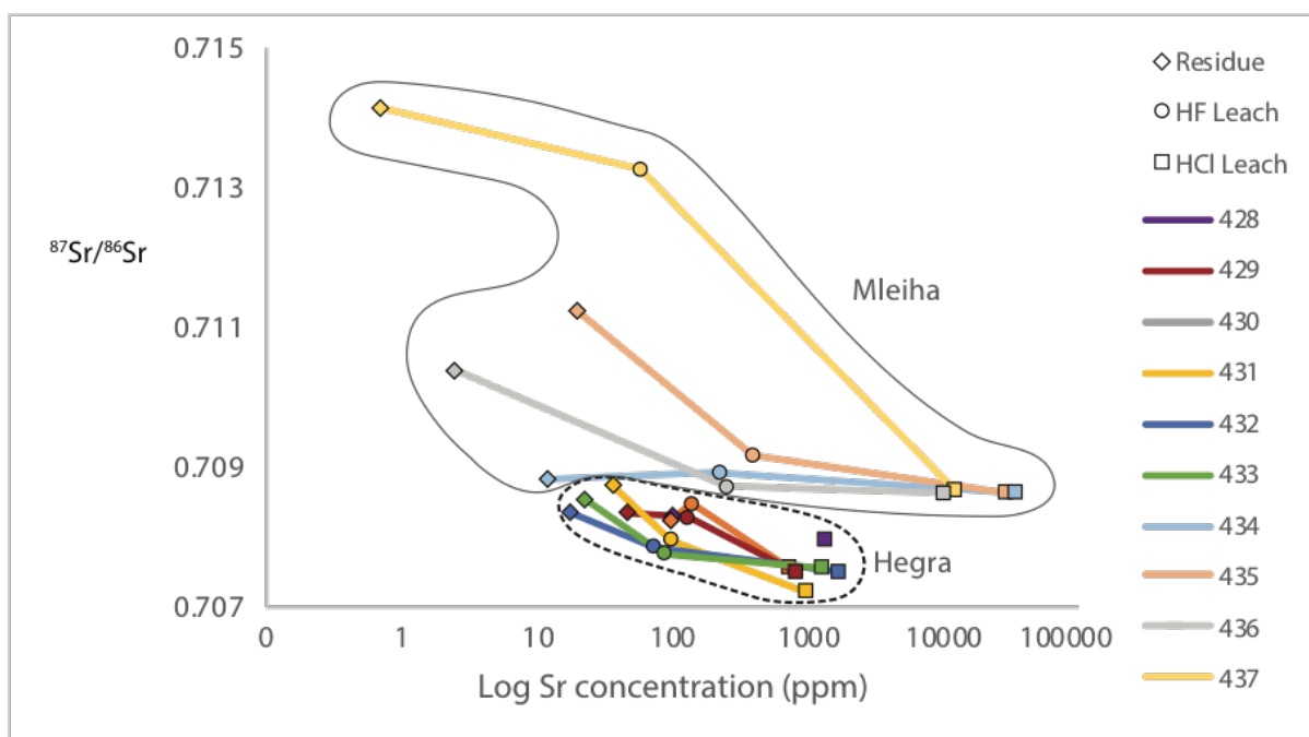
Figure S11. Strontium isotopes of the cotton textile leachates and residues, 4% uncertainty.
