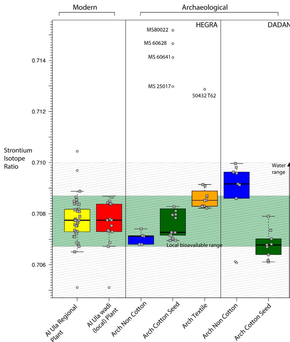
FIGURE 2 Comparative of strontium isotopes of modern plants, archaeological non-cotton plants (barley grain, date palm seed and charcoal, tamarisk charcoal, Amaranthaceae charcoal), cotton seeds, cotton textiles and groundwater. Circles indicate boxplot outliers.
