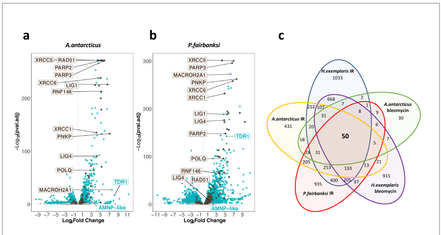
Figure 4. Transcriptomic response of A. antarcticus and P. fairbanksi to ionizing radiation (IR). (a) and (b) volcano plots representing \text{Log}_2 Fold Change and adjusted p-value ( -\log_{10} of RNA levels after irradiation with 1000Gy \gamma -rays between irradiated A. antarcticus and untreated controls ( n=3 ) (a) and between irradiated P. fairbanksi and untreated controls ( n=3 ) (b). Blue dots represent transcripts with an adjusted p-value < 0.05 . Brown dots indicate transcripts of DNA repair genes (based on KEGG DNA repair and recombination gene group ko03400) with an adjusted p-value < 0.05 . Brown labels indicate representative strongly upregulated genes of DNA repair. Blue labels indicate two tardigrade-specific genes induced in response to IR: the TDR1 gene identified in this work, and the AMNP-like gene (BV898_10264), a member of the family of AMNP/g12777-like genes upregulated in response to desiccation and UVC (Yoshida et al., 2021). (c) Venn diagram showing upregulated genes with an adjusted p-value < 0.05 common to the transcriptomic response to IR in the three species analyzed and to Bleomycin in H. exemplaris and A. antarcticus .
