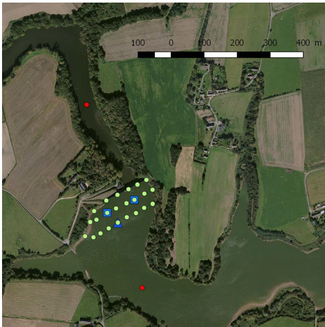
FIGURE 3 Location of the acoustic receivers with millisecond accuracy (green points) used to obtain accurate positions, and those without millisecond accuracy (red points) used to monitor the downstream or upstream movement of eels in Bois Joli Reservoir. Blue squares represent the location of the two test transmitters and blue triangle represents the position of the synchronization transmitter (ST) and reference receiver
