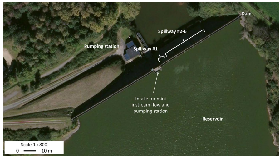
FIGURE 1 Details of the study site: In the vicinity of the dam
