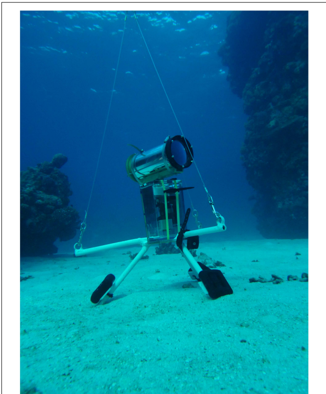
FIGURE 1 | The STAVIRO lander on a sandy bottom in New Caledonia. Credits: B. Preuss – Ifremer AMBIO project.
