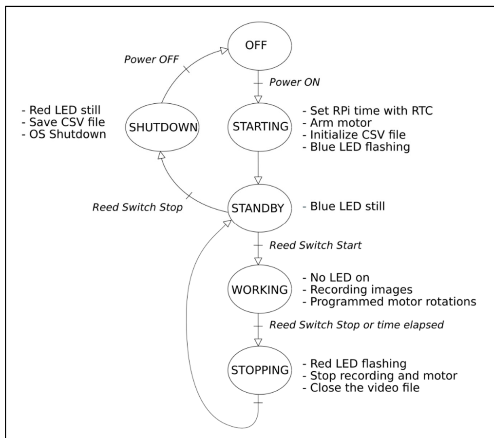
Figure 8. Flowchart of the recording process.
