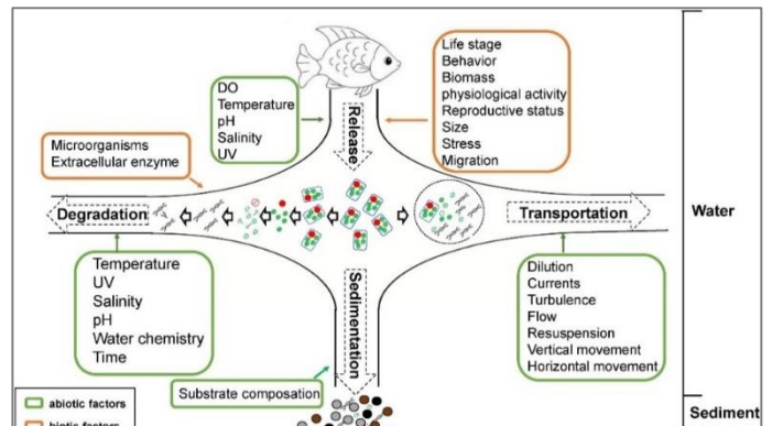
Figure 2: Schematic diagram illustrating the known associations of various influencing factors (biotic and abiotic) and the basic processes and fates (source : https://www.sciencedirect.com/science/article/pii/S0048969720361519 )
