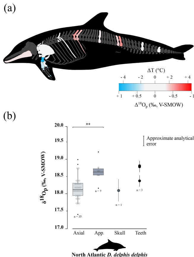
Figure 1. (a) Oxygen isotope variability within the skeleton of a North Atlantic D. delphis delphis (M.1162). Bone \Delta^{18}O_p corresponds to the difference between bone \delta^{18}O_p value and an average value of the skeleton expressed as its mid-range value ( (\delta^{18}O_{\max} - \delta^{18}O_{\min})/2 ). For paired skeletal elements as well as vertebrae centra and neural spines, the mean value is used. (b) Boxplots showing the \delta^{18}O_p values of skeletal regions for a North Atlantic D. delphis delphis . Asterisks indicate the significance of the observed differences between pairs of groups (** for p < 0.01 ). Outliers are plotted as small black circles. Abbreviation: App. (appendicular skeleton).
