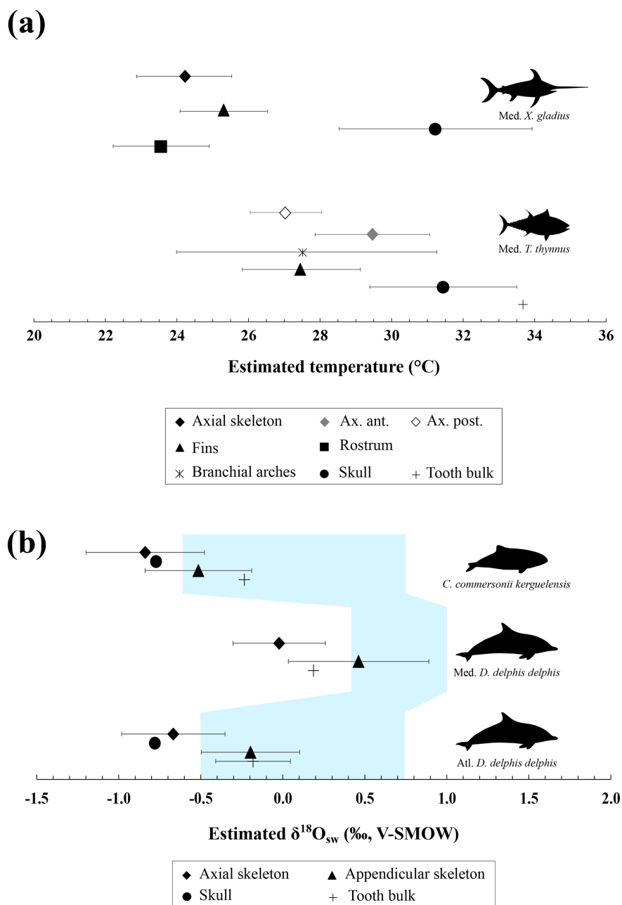
Figure 3. (a) Mean estimated hydroxylapatite mineralisation temperature from the phosphate–water oxygen fractionation equation published by Lécuyer et al. (2013), where body water oxygen isotope composition ( \delta^{18}\text{O}_{\text{bw}} ) for osteichthyans is assumed to be equal to the \delta^{18}\text{O}_{\text{sw}} value. Temperature estimates were done with the mean annual oxygen isotope composition of the Mediterranean Sea ( \delta^{18}\text{O}_{\text{sw}} = 1.5 \pm 0.4\text{‰} ; Table S5). Error bars correspond to 1 SD. (b) Mean estimated \delta^{18}\text{O}_{\text{sw}} from the phosphate–water oxygen fractionation equation for cetaceans published by Ciner et al. (2016). Error bars correspond to 1 SD and the shaded blue form corresponds to the real measured \delta^{18}\text{O}_{\text{sw}} values (LeGrande and Schmidt, 2006). Abbreviations: Med. (Mediterranean Sea), Atl. (Atlantic Ocean).
