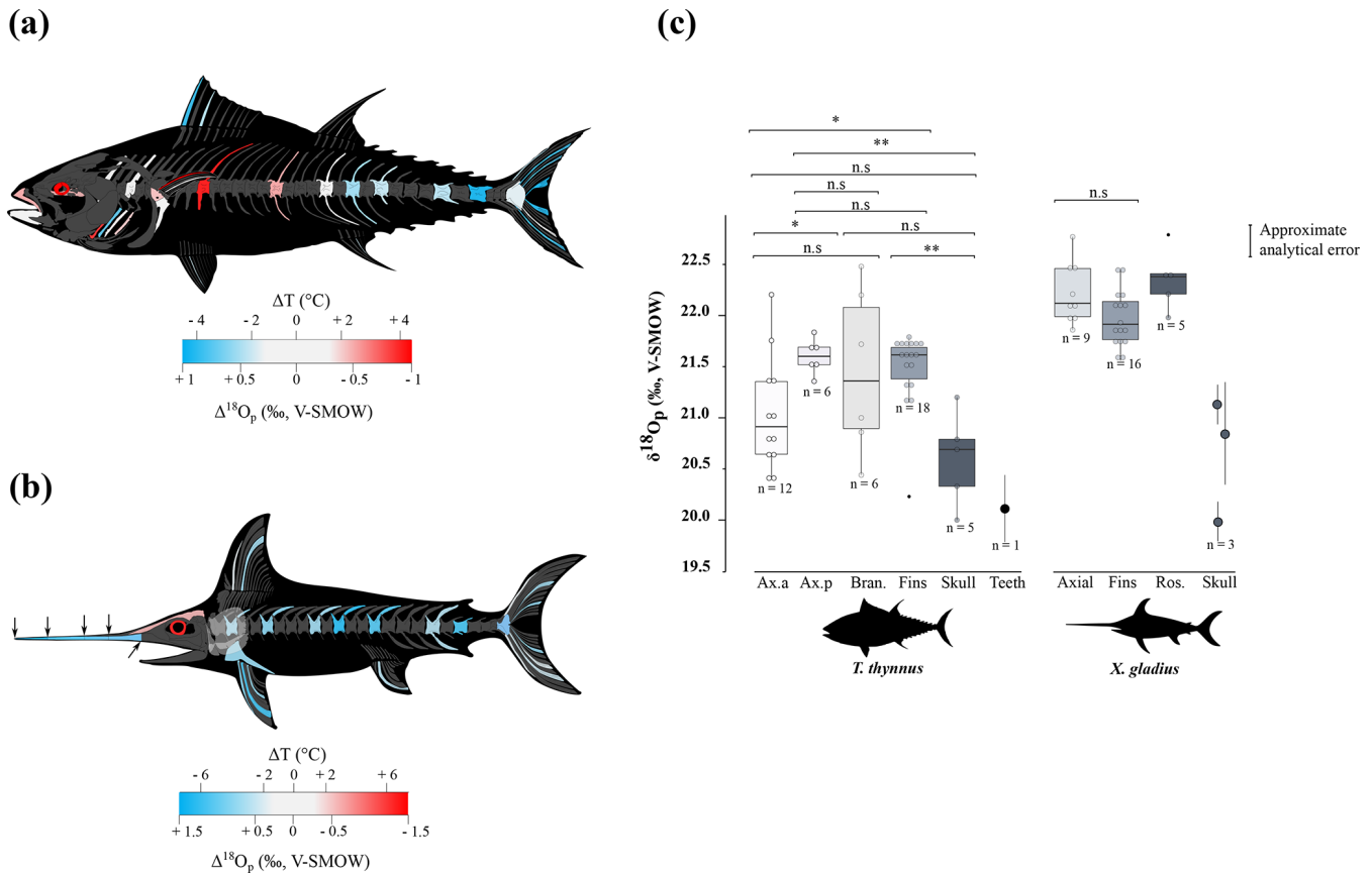
Figure 2. Oxygen isotope variability within the skeleton of T. thynnus (a) and X. gladius (b). For each specimen, bone \Delta^{18}\text{O}_p corresponds to the difference between bone \delta^{18}\text{O}_p value and an average value of the skeleton expressed as its mid-range value ( (\delta^{18}\text{O}_{\text{max}} - \delta^{18}\text{O}_{\text{min}})/2 ). For paired skeletal elements, as well as vertebrae centra and neural spines and fin spines and rays, the mean value is used. The arrows represented on the swordfish's skull represents the precise location of the sampling. (c) Boxplots showing the \delta^{18}\text{O}_p values of skeletal regions for T. thynnus and X. gladius . Asterisks indicate the significance of the observed differences between pairs of groups: ns (not significant) for p > 0.05 , * for p < 0.05 , ** for p < 0.01 (highly significant difference). Outliers are plotted as small black circles. Abbreviations: Ax.a (axial anterior), Ax.p (axial posterior), Bran. (branchial arches), Ros. (rostrum).
