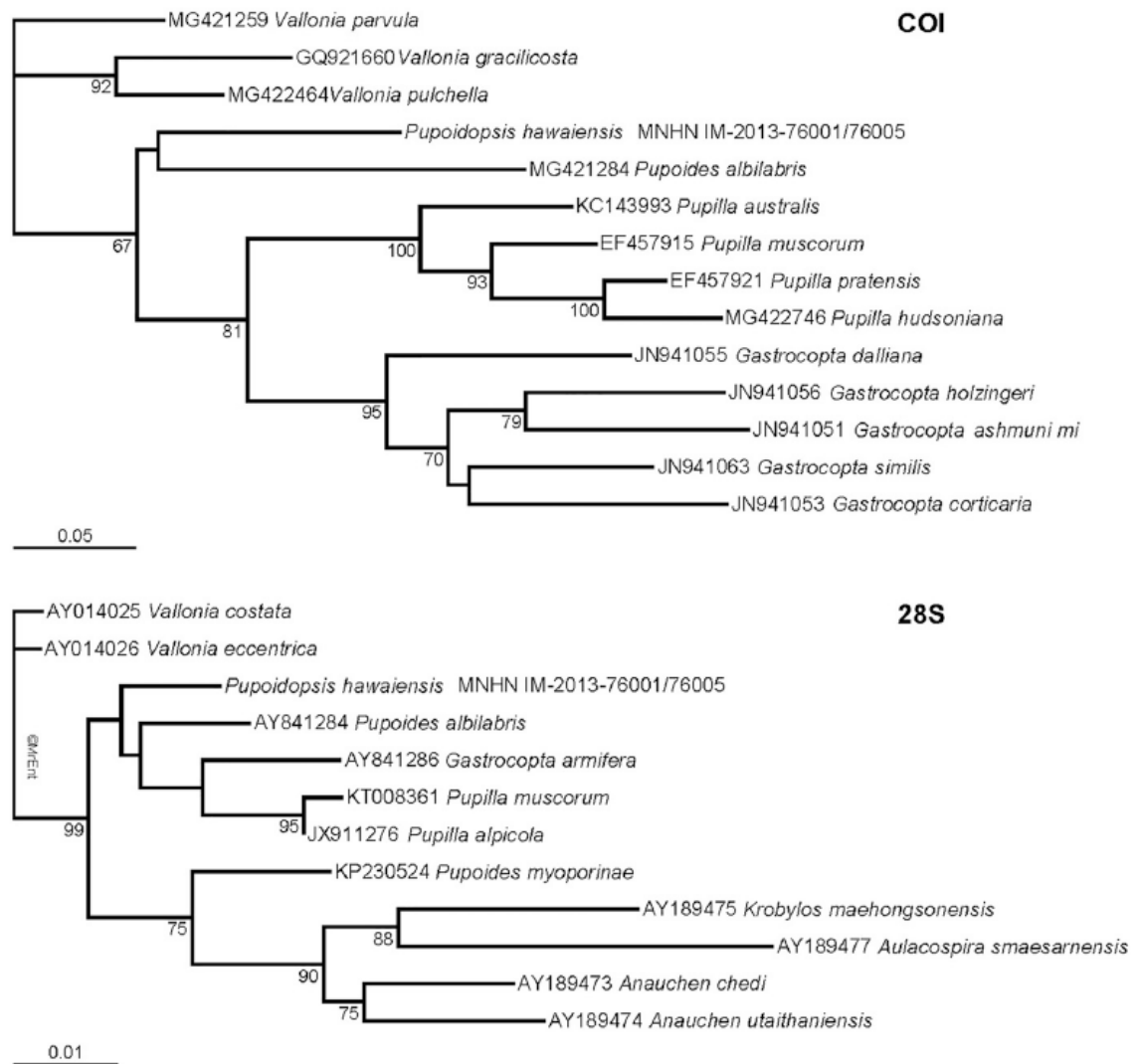
Figure 4. Maximum-likelihood trees based on COI (top) and 28S sequences (bottom). The bootstrap support values (>50%) are indicated at the node.
