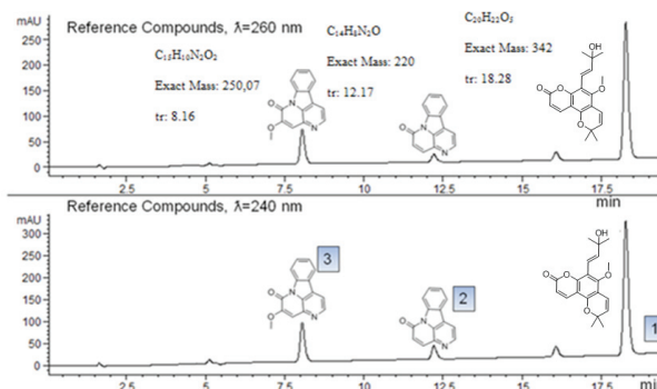
Figure 1. HPLC-UV Chromatogram of reference compounds ( \lambda=260 and 240 nm).
