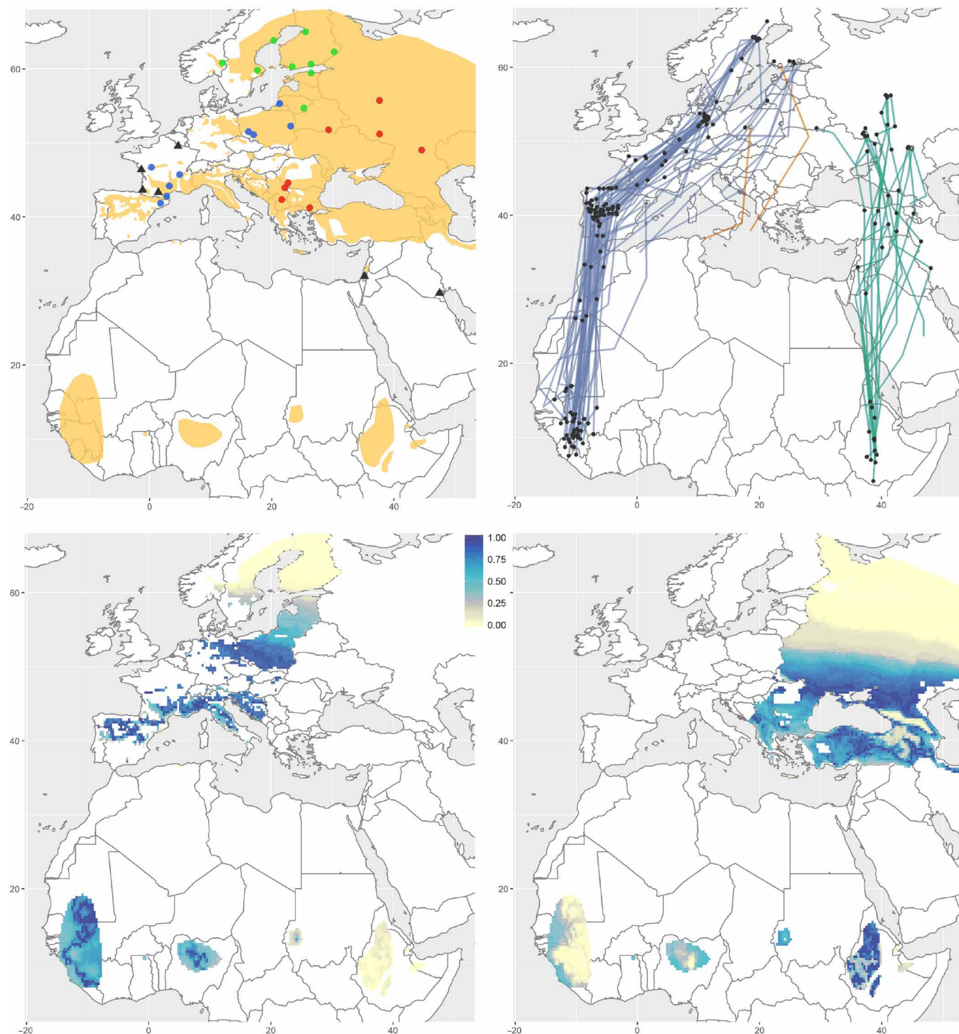
Fig. 1. Range, genetic population structure, and migration flyways of European ortolan buntings Emberiza hortulana as revealed by light loggers and stable isotopes.
