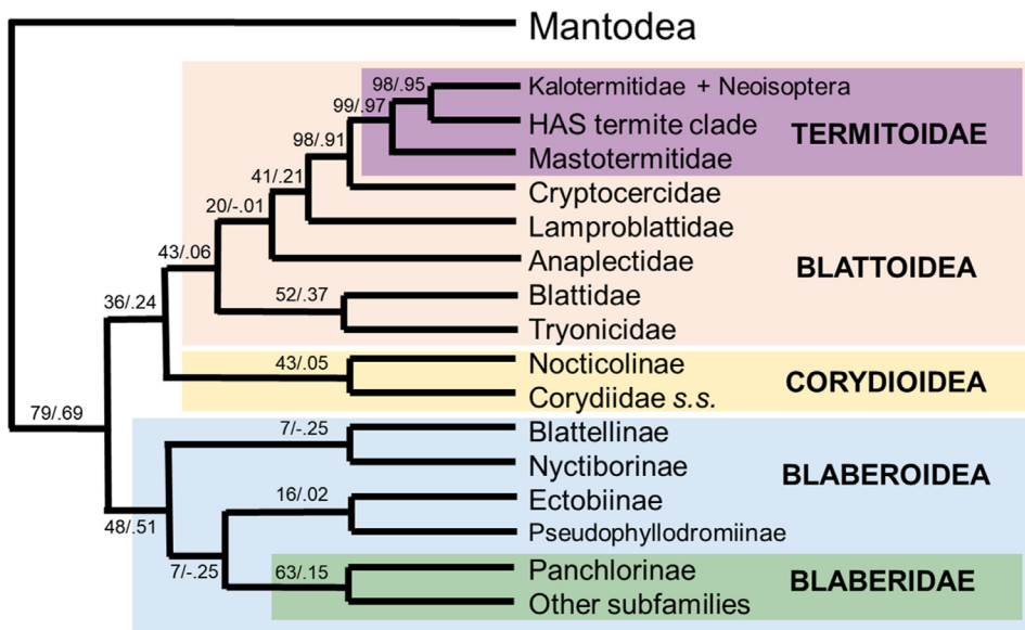
Fig. 2. Focal tree topology (1geneMin tree) for major lineages in Blattoidea and support. Tree was inferred in RAXML from molecular data for six loci obtained for 575 taxa. Support values are bootstrap frequencies and internode certainty values. We see strong support for the monophyly of Blattoidea, Blaberoidea, termites + Cryptocercidae, and termites; moderate support for Lamproblattidae + Cryptocercidae + termites, Tryonicidae + Blattidae, and Blaberidae; low support for Anaplectidae + sister group, Blattoidea, Corydioidea, and most relationships in Blaberoidea. Full tree with support values is available in Appendix D . See Fig. 1 caption for family-name usages.
