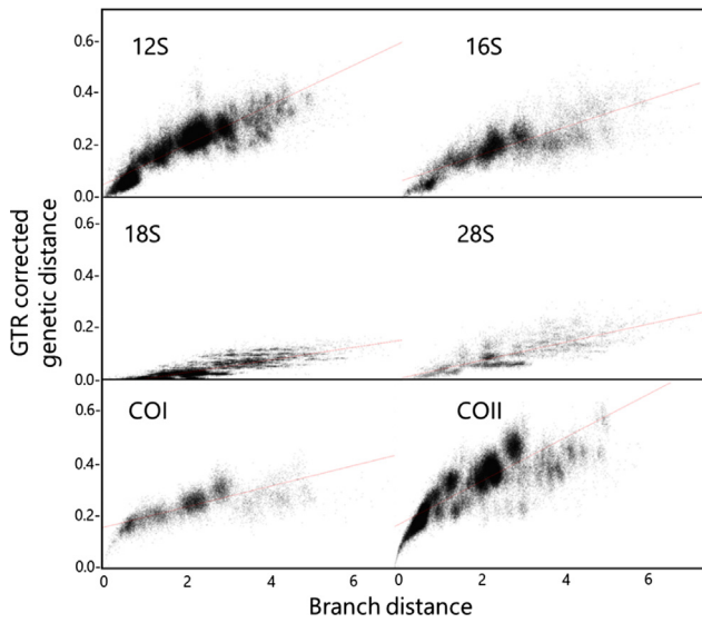
Fig. 5. Locus saturation per time-scale. Pairwise branch distance on the horizontal axis plotted against pairwise GTR model corrected distance on the vertical axis. Trend lines calculated from a best fit linear regression. Equations for each trend line are as follows: 12S, 0.048 + 0.077x ; 16S, 0.063 + 0.053x ; 18S, -0.019 + 0.023x ; 28S, 0.01 + 0.035x ; COI, 0.155 + 0.040x ; COII, 0.160 + 0.084x . Plots show that 18S and 28S are more conserved at all ages and have phylogenetic utility at deep phylogenetic scales. 16S and COI are moderately fast evolving. 12S and COII are the least conserved and may be limited in their use at deep phylogenetic scales.
