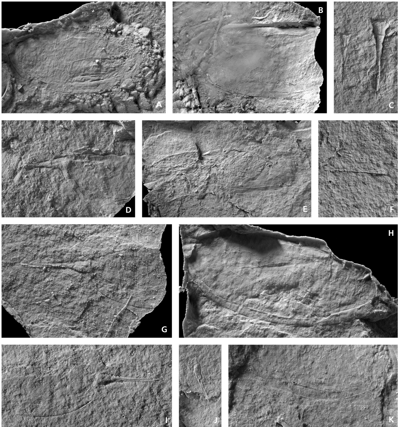
Figure 14. Rolfecaris lethiersi gen. et sp. nov. Agua Blanca section (type locality) sample 7 of Blanca Toro. All figures are latex casts. All specimens \times 5 . • A – incomplete left valve of the carapace with proximal part of the tail piece still attached, holotype No. 23259. • B – incomplete right valve, No. 23346. • C – two isolated telson, No. 23258. • D – posterior part of an incomplete right valve with telson still articulated, No. 23257. • E – right valve, No. 23240. • F – isolated telson, No. 23254. • G – posterior part of an incomplete right valve with telson still articulated, No. 23262. • H – large right ventral valve, No. 23255. • I – posterior part of a left valve with articulated telson, No. 23261. • J – small isolated telson, No. 23260. • K – ventral margin of an incomplete right valve, No. 23264.
