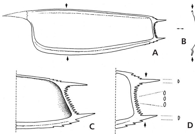
Figure 4. Janviericaris formosa sp. nov. Reconstructed inner side of a right valve showing the outline of the inner border (A) with the corresponding cross section (B); arrows indicate the location of the cross section. • C – hypothetical anteroventral view of the inner posterior part of the carapace. • D – enlarged view of the posterior margin of the carapace with cross sections of spines; note the elliptical section of the small posterior spines and the sub-semicircular cross section of posteroventral and posterodorsal spines. Pre-posteroventral and pre-posterodorsal spines are well developed.
