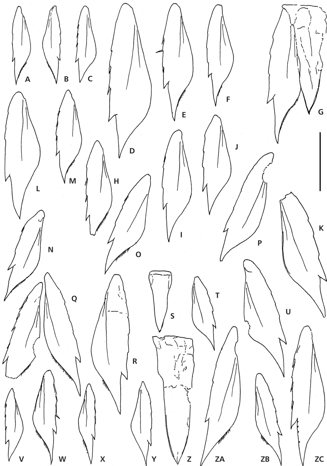
Figure 10. Janviericaris jujuyensis sp. nov. furcal rami, telsons and tailpieces from Los Colorados (A–K), La Luna (L–O), and Mina Natasia (localities 3–4) (P–ZC) sections. • A–F – No. 23274–23279, 23285, and 23286–23288, respectively. • L–O – No. 23280, 23281, 23283, and 23284, respectively. • Q–ZC – No. 23311, 23312, 23300, 23298, 23305, 23316–23318, 23314, 23313, 23315, 23299 and 23297. Scale bar = 5 mm.
