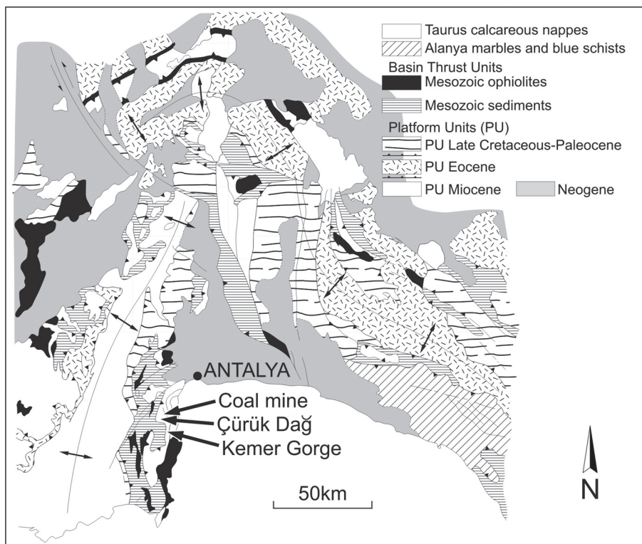
Fig. 1 - Geological sketch map of the Western Taurus showing the location of the Çürük Dağ composite section at N36°41'32"-E30°27'40", 1425 m a.s.l.
