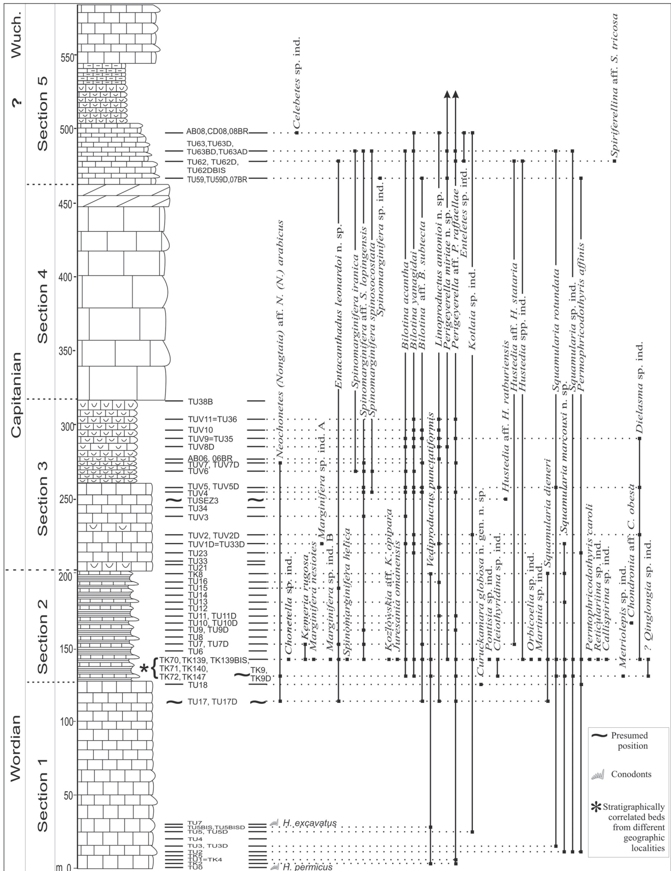
Fig. 4 - Detailed composite log of Çürük Dağ showing the distribution of brachiopods from section 1 to section 5.
