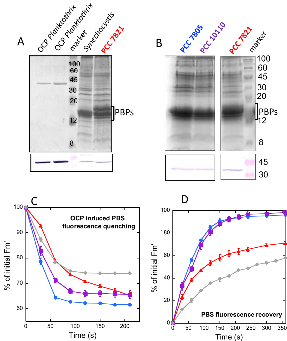
Fig. 2. The OCP and the related photo-protective mechanism. (A and B) Gel electrophoresis and OCP detection by anti- Synechocystis OCP. (A) isolated Planktothrix PCC 7805 OCP (slots 1 and 2, 0.5 and 1 \mu\text{mol} respectively); (slots 3–4) isolated membrane-bound phycobilisome complexes of Synechocystis PCC 6803 (3) and Planktothrix PCC 7821 (4). (B) total cell protein of Planktothrix PCC 7805, Planktothrix PCC 10110 and Planktothrix PCC 7821. The cells for these experiments were grown at 20 \mu\text{mol photons m}^{-2} \text{s}^{-1} (C and D) PBS fluorescence quenching induced by strong blue light (1200 \mu\text{mol photons m}^{-2} \text{s}^{-1} ) in Planktothrix cells grown at 20 \mu\text{mol photons m}^{-2} \text{s}^{-1} (C) and fluorescence recovery under low blue light was measured by a 101/102/103-PAM (Walz, Effeltrich, Germany) with 650 nm detecting light (D). Planktothrix PCC 7805 (blue circles), PCC 10110 (violet squares), PCC 7821 (red triangles) and Synechocystis PCC 6803 (gray diamond).
