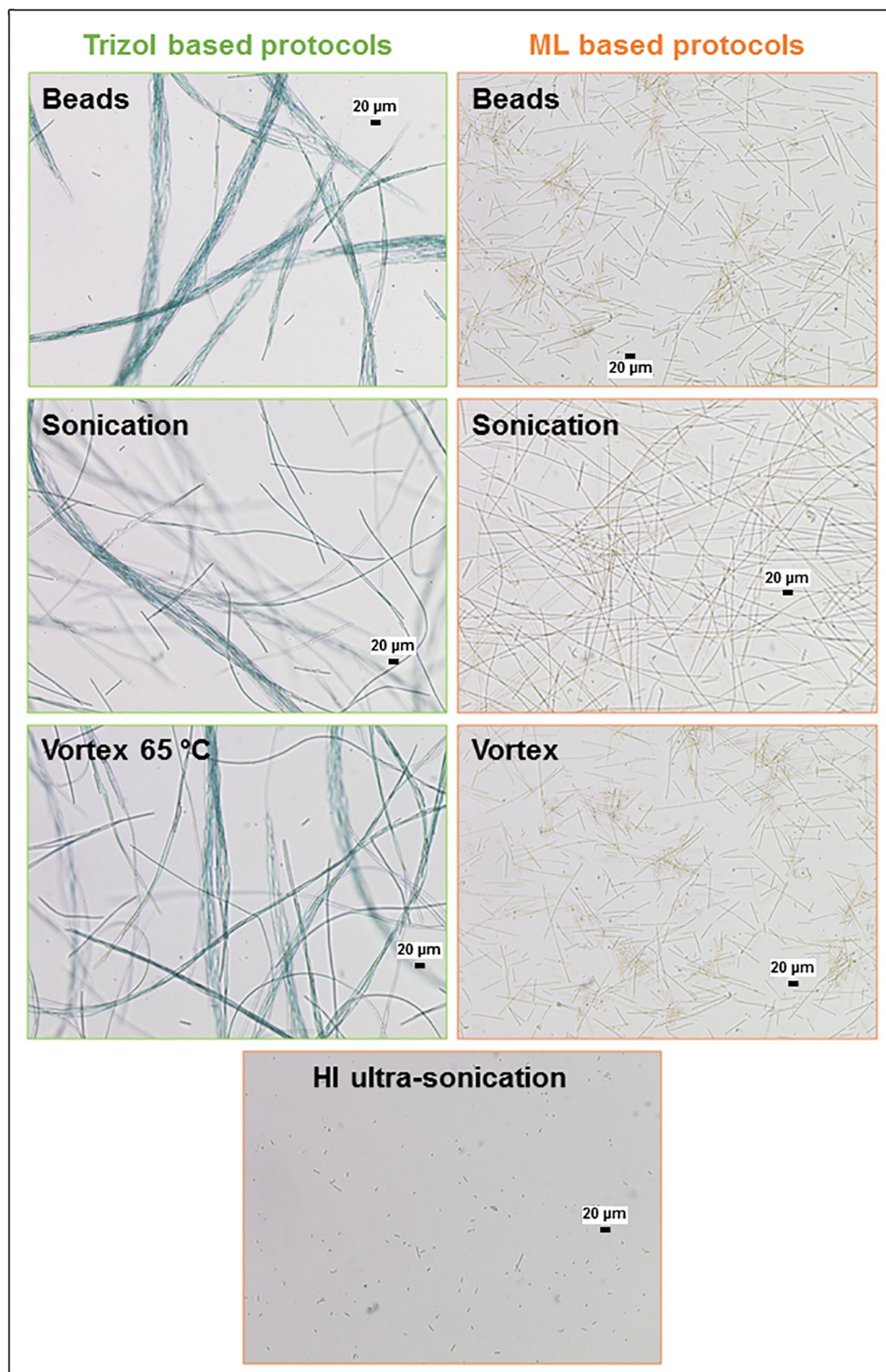
Fig 2. Microscopic observations (n = 2) of P. agardhii after “Beads,” “Sonication,” “Vortex 65,” and “HI ultra-sonication” RNA extraction protocols realized in Trizol or Lysis buffer ML.
