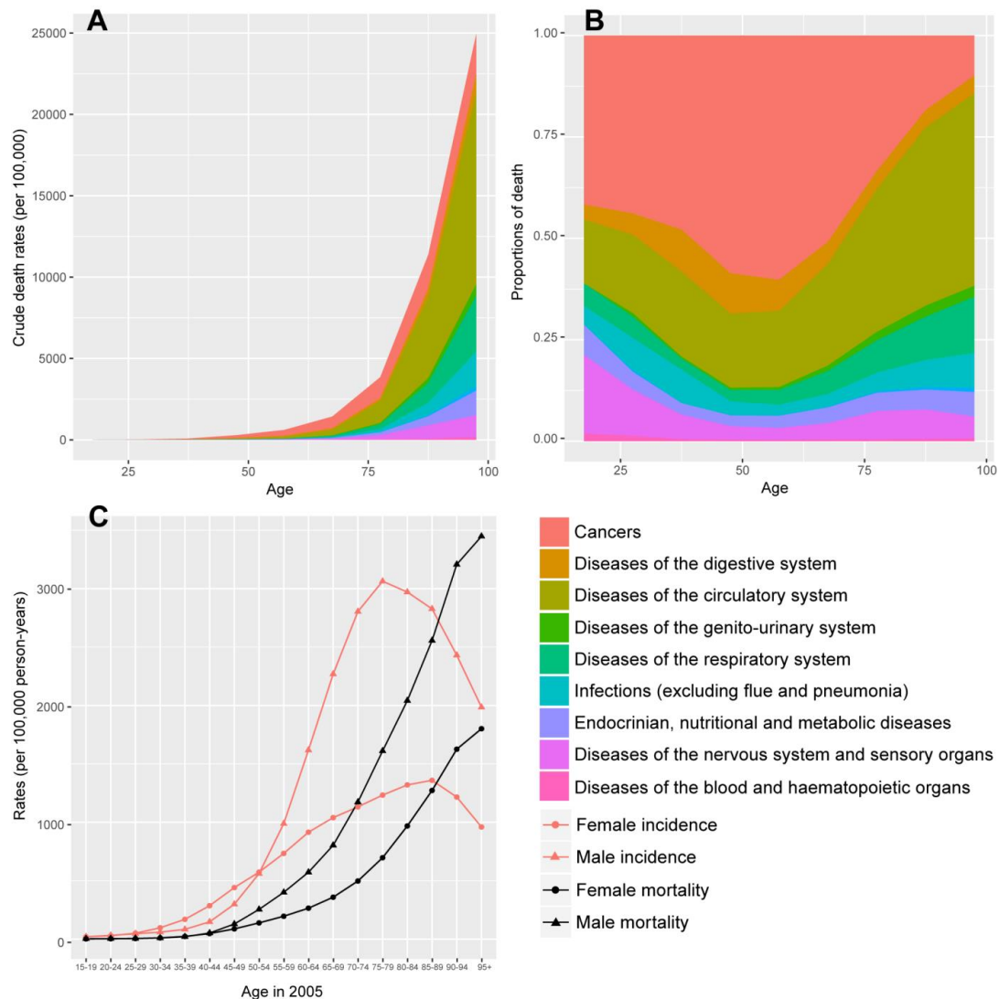
Figure 3 - Stacked crude death rates (A) and proportions of death (B) per causes in France in 2005. Data were gathered by the 'Centre d'épidémiologie sur les causes médicales de décès' de l'Institut national de la santé et de la recherche médical (Inserm-CépiDc). Data, data documentation, and methods for death rates calculation can be found here http://www.cepidc.inserm.fr/ . Panel (C) shows sex-specific incidence and mortality by cancers by age in 2005 France. Figure is reproduced from Bélot et al. (2008); where exceptionally detailed data on cancer incidence per site can also be found.
