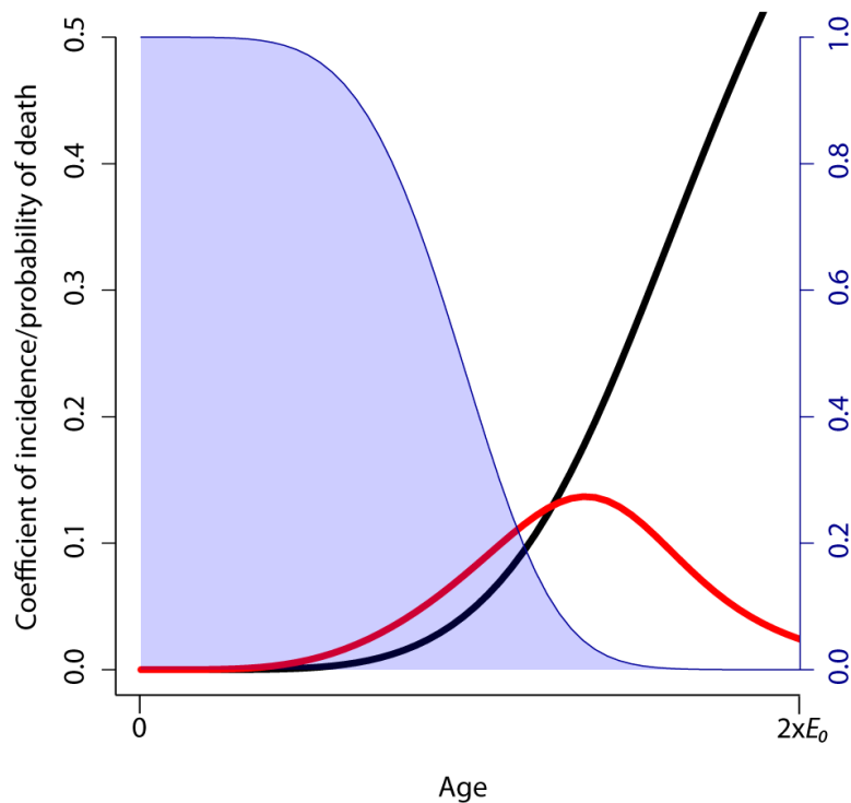
Figure 4 – Incidence of cancer (red) and probability of death resulting from the accumulation of senescent cells (black) for an optimal accumulation of senescent cells by time-step of \sigma^* = 0.05 for parameters \Phi = 500 , r_{CS} = 2.5 , r_{OS} = 2 and r_{OT} = 2.6 . In this case E_0(\sigma^*) = 27 .
