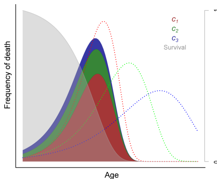
Figure 1 - Stacked distributions of deaths f_c(t) = S_1(t)S_2(t)S_3(t)h_c(t) across age t for three causes of death c_1 , c_2 and c_3 (red, green and blue polygons, respectively); the corresponding overall survival over age S(t) = S_1(t)S_2(t)S_3(t) (grey polygon and right axis); as well as the distribution of death from each cause f_c(t) = S_c(t)h_c(t) in the case where individuals die from only this cause (red, green, and blue dotted lines). In this example, cause-specific mortality hazards are Gompertz-shaped (such that h(t) = ae^{b_c t} , with a=0.001 , b_1=0.1 , b_2=0.07 and b_3=0.05 ).
