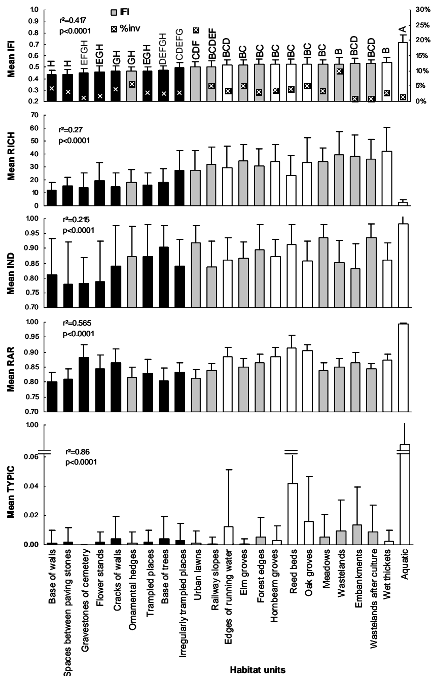
Fig.2. Mean values of floristic interest variables across habitats (Rich: species richness, Typic: proportion of typical species, Ind: proportion of indigenous species, Rar: mean rarity index and IFI: Index of Floristic Interest) and percentage of sites inventoried for each habitat (%inv, top figure). Significant differences ( p=0.05 ) between IFI values are shown by different letters (Tukey's test). Semi-natural habitats are in white, intermediate habitats in grey, and anthropogenic habitats in black.
