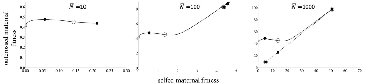
9 Figure 3: Relationships between maternal selfed and outcrossed components of fitness under the 10 random rank visitation model with pollinator attraction limitation ( a = 50 , b = 0.1 ) and 11 pollinator abundance limitation ( M = 10 and \tau = 0.33 ), for \rho = 0.25 , A = 100 , and three 12 values of total number of flowers per plant, \bar{N} . Edge (squares) and internal (circles) stable (full) 13 or unstable (open) equilibria, with minor internal equilibria on the dashed lines. Other parameters 14 U = 0.2 and d = 0.25 .
